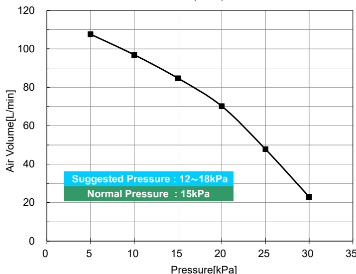
Performance Curve MAC80R (60Hz)
