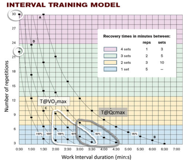
Fig. 6 'Thibault' graphical model [150]. All particular high-intensity interval training sessions ( black dots ) are obtained while manipulating work interval duration ( x axis ) and the number of repetitions ( y axis ). All sessions are (empirically) believed to represent a similar overall exercise strain, based on empirical observations with respect to the rating of perceived exertion responses (see Part I, Sect. 2.4 [1]). The black lines join the different sessions performed at a similar percentage of the minimal velocity/power associated with maximal oxygen uptake ( v/p \dot{V}O_{2max} ). For a work interval of 95 % of v/p \dot{V}O_{2max} for example, if 3 intervals are performed, the suggested interval duration of each is 3 min 30 s, if 4–5 intervals are performed, then 3 min each, if 6–7 intervals are performed, then 2 min 30 s each, etc. The number of series needed to perform a given number of repetitions is provided in the table, together with the between-series recovery duration. As an example, the two small white circles on the y axis illustrate two high-intensity interval training sessions (i.e. 22 \times 1 min 30 s at 110 % and 30 \times 2 min at 105 % of v/p \dot{V}O_{2max} ) believed to be identical with respect to RPE. The large white-circled zone illustrates the maximized high-intensity interval training formats with respect to time spent at maximal oxygen uptake ( T@ \dot{V}O_{2max} ) and the grey-circled zone illustrates the maximized high-intensity interval training formats with respect to time spent at maximal cardiac output ( T@ Q_{cmax} ) (Part I [1]). Reproduced from Thibault [150], with permission
