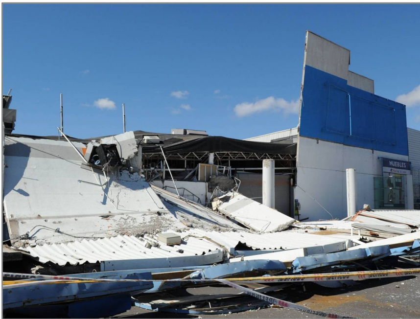
Figure 2-8 – Collapse of tilt-up walls, 2010 Chilean Earthquake
