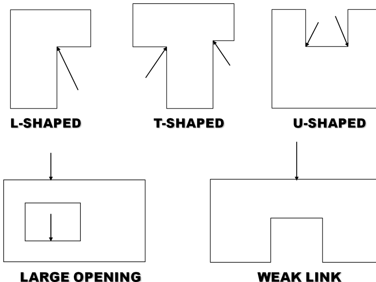
Figure 2-32 – Plan Irregularities
