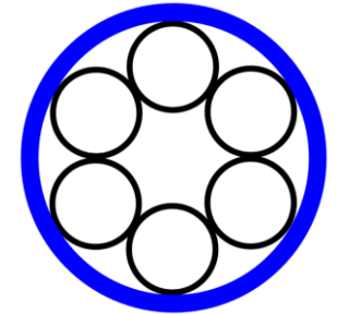
Method 3
