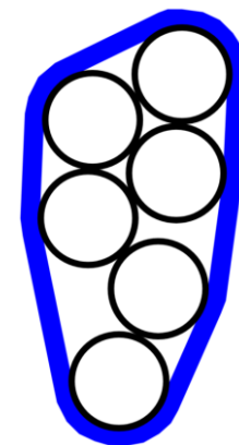
Method 4
