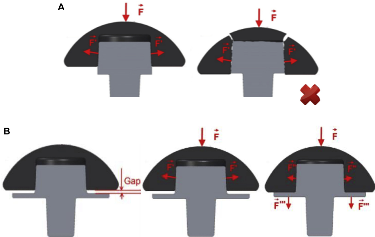
Figure 7 The Aequalis Ascend Flex pyrocarbon humeral head is created by combining a pyrocarbon bearing surface and a cobalt-chromium (CoCr) double taper neck. The pyrocarbon bearing surface is assembled on its CoCr double taper neck in the factory. No breakage of the Aequalis Ascend Flex pyrocarbon humeral head has occurred since its launch on the market in 2013. (A) A classical Morse taper cannot be used with a pyrocarbon head because of its low Young modulus and poor resistance to traction: When applying a force of impaction ( F ), the risk of breakage of the pyrocarbon is too high. (B) To make the Morse taper reliable and safe, an abutment is added to stop the pyrocarbon bearing surface translation at an appropriate level. The addition of a metallic plate (1.5 mm in thickness) allows division of the force ( F ) into 2 parts: F'' and F''' . Before mounting, there is a gap between the pyrocarbon head and the metallic plate. At the beginning of assembly, the force F'' is enough to keep the pyrocarbon bearing surface in place (pullout and torque-out strength) but remains under the limit of breakage of graphite and pyrocarbon in traction. At the end of assembly, the force F''' is transmitted through the head to the metallic plate, which is a CoCr alloy and provides resistance.
