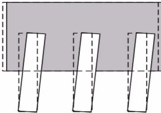
(a) Rotation of piles within cap
